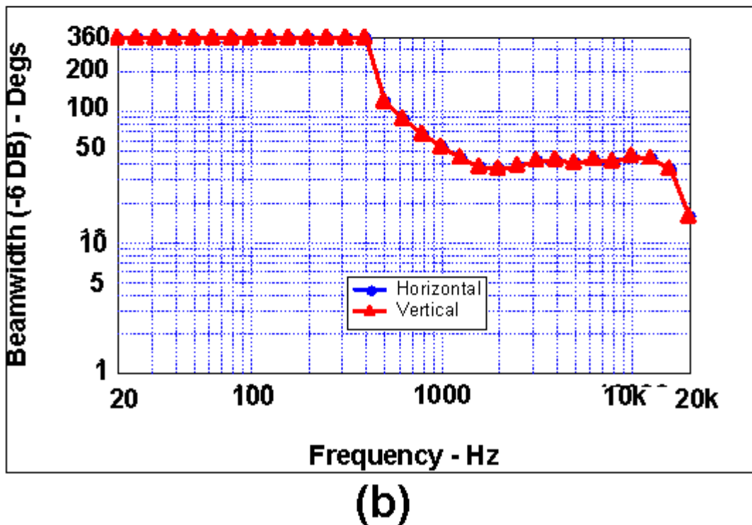
Fig. 21. (a) Source configuration and (b) beamwidth vs. frequency of the delay-derived circular flat-panel CBT array designed for 40° coverage with a 62.5° cap (arc) angle of Fig. 20. Compare with the conventional CBT array data of Fig. 15.
