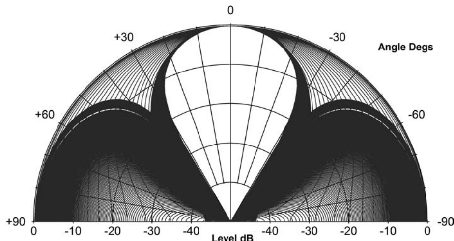
Fig. 10. Cylindrical composite polar plot for constant-beamwidth array that provides a rounded-shape beam. Polar radial range is 50 dB with 10° angular increments.
