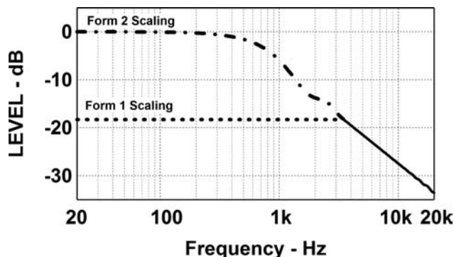
Fig. 2. Normalized far-field on-axis frequency response for constant-aperture constant-beamwidth straight-line array that provides a wedge-shaped beam. Array maintains constant-beamwidth operation only above 3.5 kHz (—) where response falls at 6 dB per octave. Form 1 scaling (•••) exhibits significant low-frequency loss (18.3 dB) compared to form 2 scaling (—•—).
