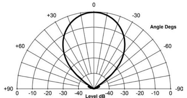
Fig. 11. Cylindrical polar plot at 6.3 kHz for constant-aperture constant-beamwidth array that provides a rounded-shape beam.
