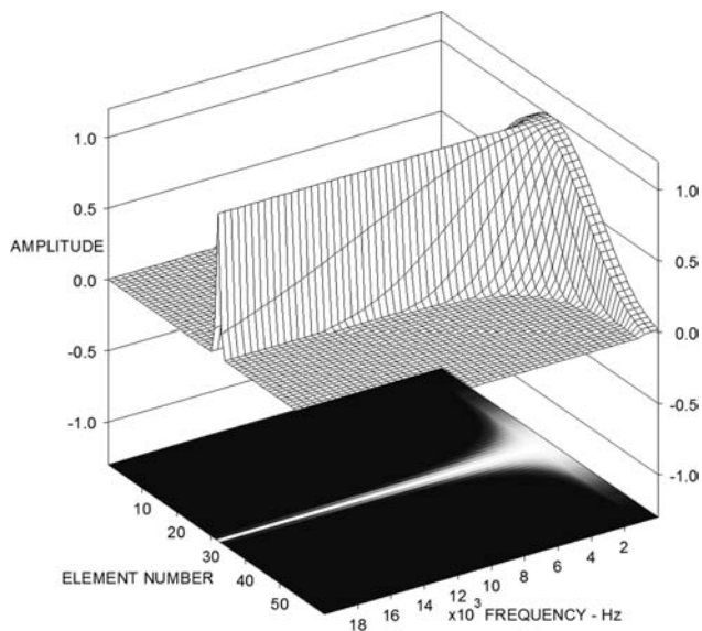
Fig. 13. Three-dimensional array coefficient plot versus frequency for constant-beamwidth array that provides a rounded-shape beam. Note that plot does not include array's flat on-axis equalization.
