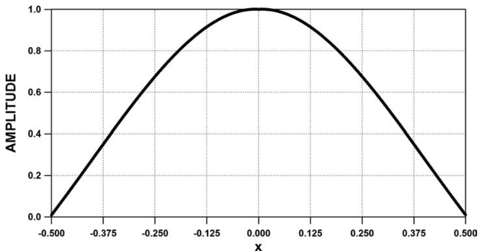
Fig. 15. Legendre window used to design a constant-beamwidth CBT array.
