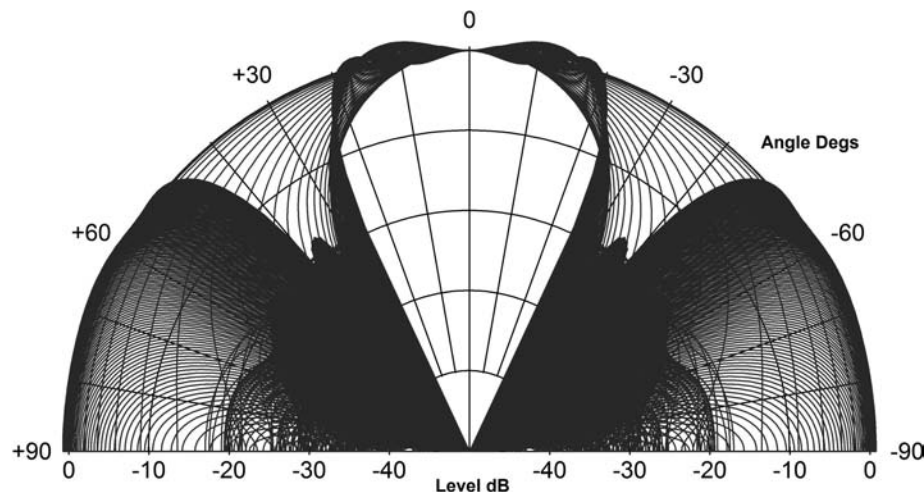
Fig. 3. Cylindrical composite polar plot for constant-beamwidth array that provides a wedge-shaped beam. Polar radial range is 50 dB with 10° angular increments.
