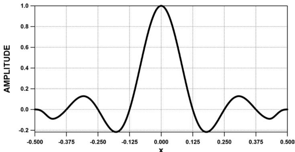
Fig. 1. Tukey-sinc window with \alpha = 0.85 and f_0 = 4 Hz used to design a constant-beamwidth straight-line array that provides a wedge-shaped beam.
