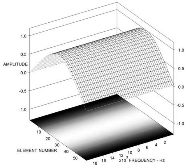
Fig. 20. Three-dimensional array coefficient plot versus frequency for constant-beamwidth curved-line CBT array. Note that plot does not include array's flat on-axis equalization and coefficients are independent of frequency.
