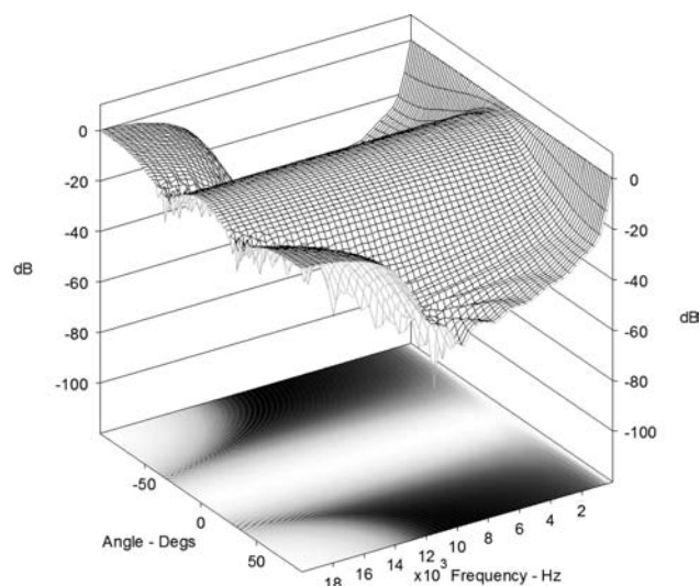
Fig. 24. Three-dimensional polar plot for constant-beamwidth straight-line CBT array with projected two-dimensional polar plot on bottom of display.
