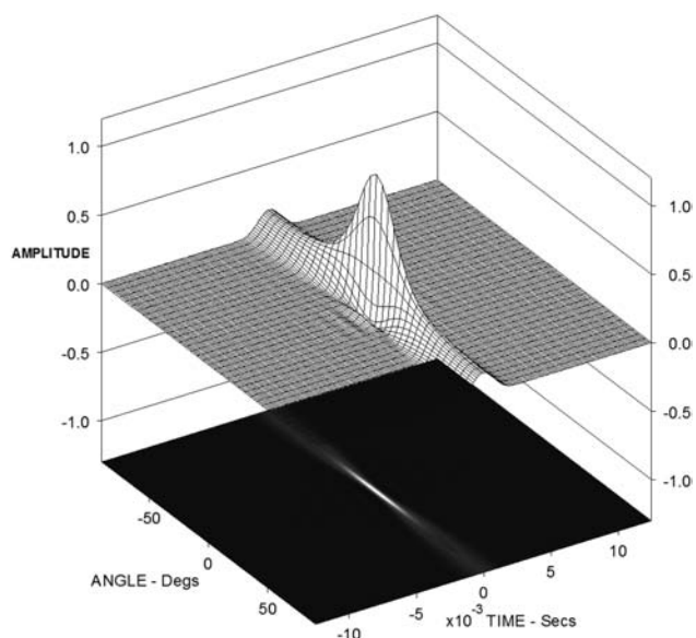
Fig. 14. Three-dimensional plot of cross correlation between on- and off-axis impulse responses for constant-aperture constant-beamwidth array that provides a rounded-shape beam.
