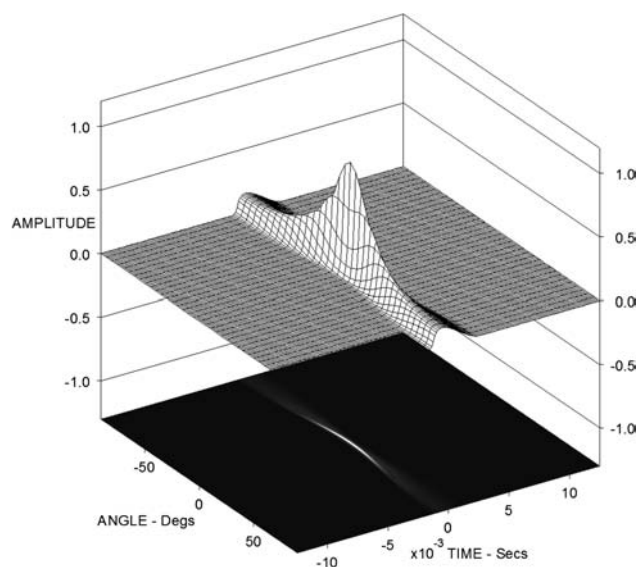
Fig. 25. Three-dimensional plot of cross correlation between on- and off-axis impulse responses for constant-beamwidth straight-line CBT array. Bottom of display shows projected two-dimensional polar plot.
