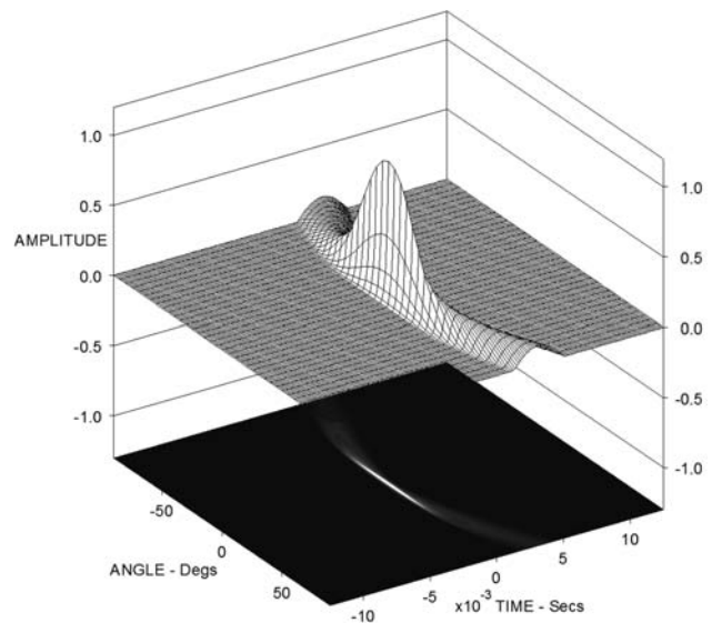
Fig. 21. Three-dimensional plot of cross correlation between on-axis and off-axis impulse responses for constant-beamwidth curved-line CBT array.
