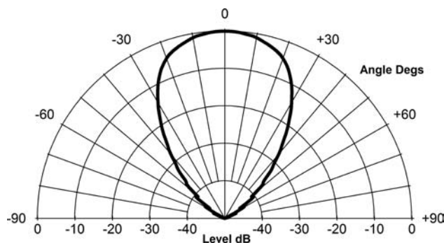
Fig. 18. Cylindrical polar plot at 6.3 kHz for CBT constant-beamwidth curved-line array that provides a rounded-shape beam.
