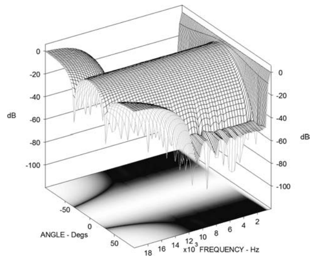
Fig. 12. Three-dimensional polar plot for constant-aperture constant-beamwidth array that provides a rounded-shape beam.
