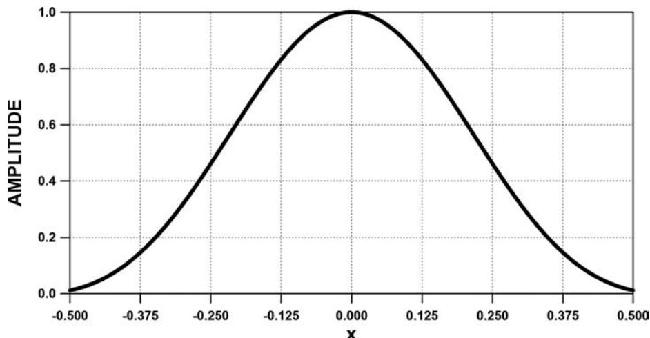
Fig. 8. Kaiser-Bessel window with \beta = 6.34 used to design a constant-beamwidth straight-line array that provides a rounded-shape beam.
